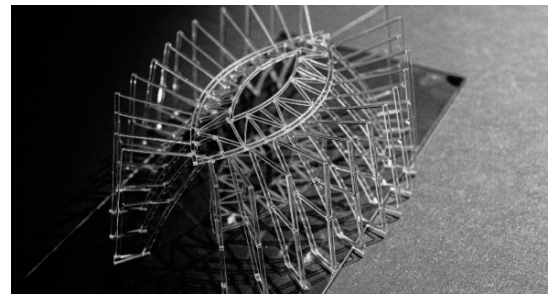
Year 1, Semester 2; SOM Cathedral of Christ the Light structural model
